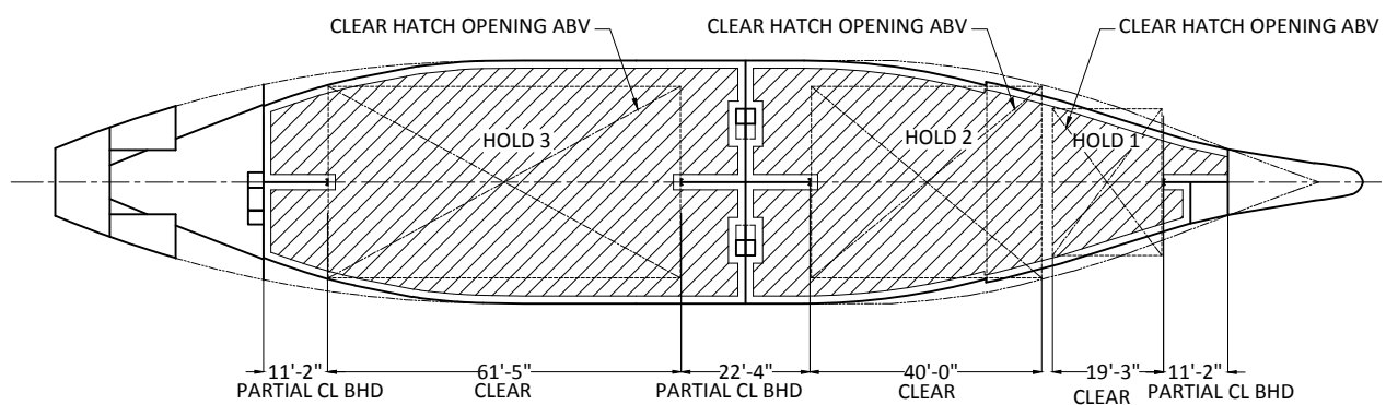
HOLD PLAN
